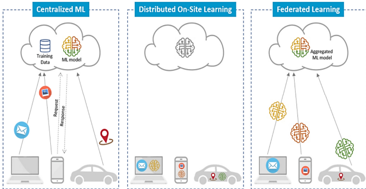
Figure 4: IDS architecture strategies
