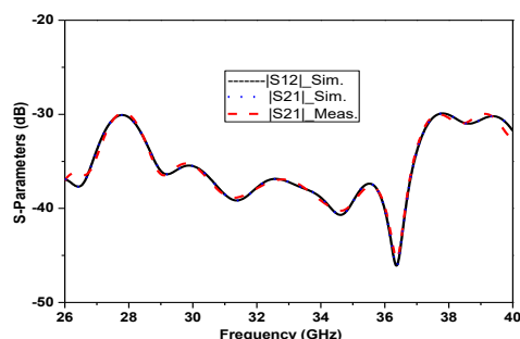
Fig.9 Transmission Coefficients for the Two Element Antenna.
